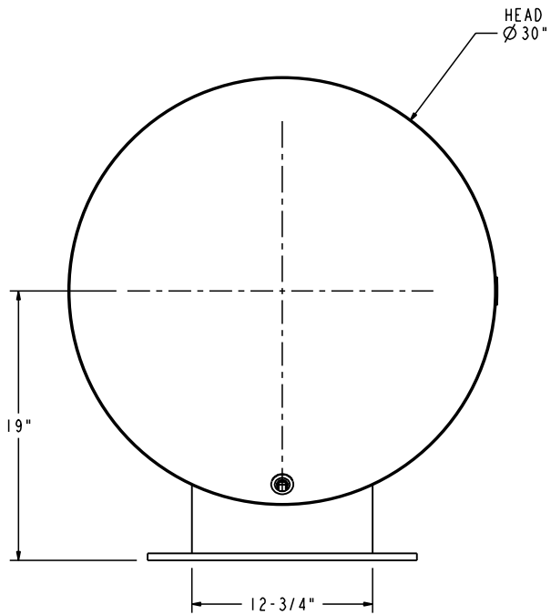
VIEW FROM INLET END
