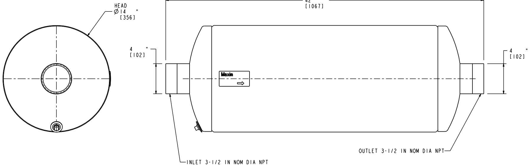
VIEW FROM INLET END
