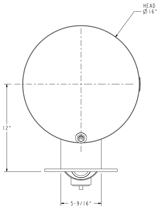
VIEW FROM INLET END
